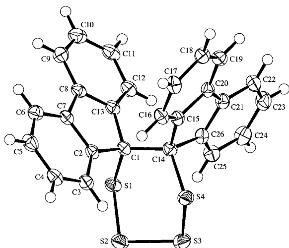
Figure 1 View of the molecule of the title compound, (IV), showing the atom-labelling scheme. Displacement ellipsoids are drawn at the 50% probability level. H atoms are represented by circles of arbitrary size.
