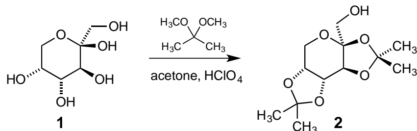
Scheme 1. Synthesis of 2,3:4,5-Di- O -isopropylidene- \beta -D-fructopyranose ( 2 ).
